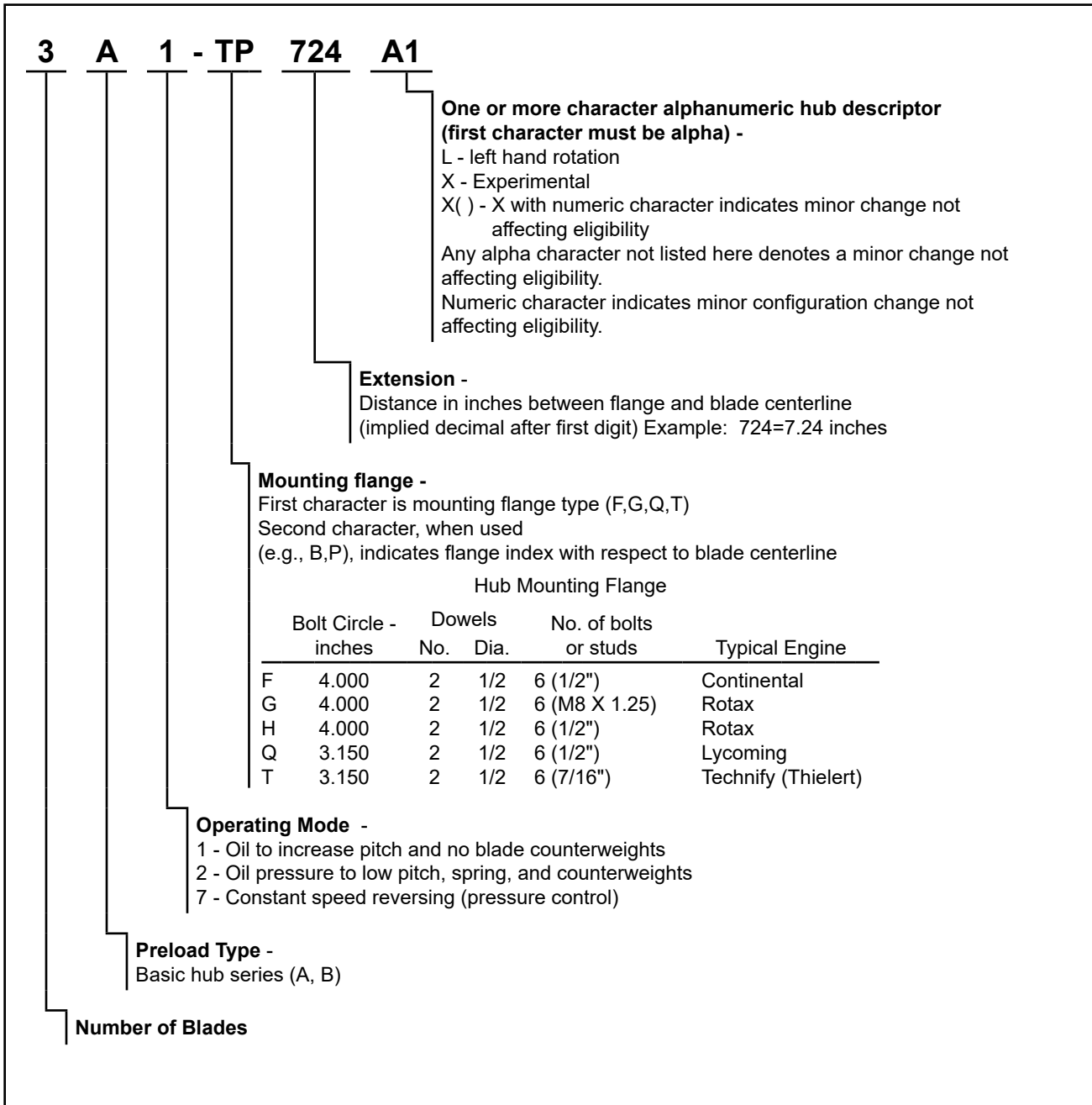
Aluminum Hub Propellers on Reciprocating Engines Identification - Bantam Series Figure 4
