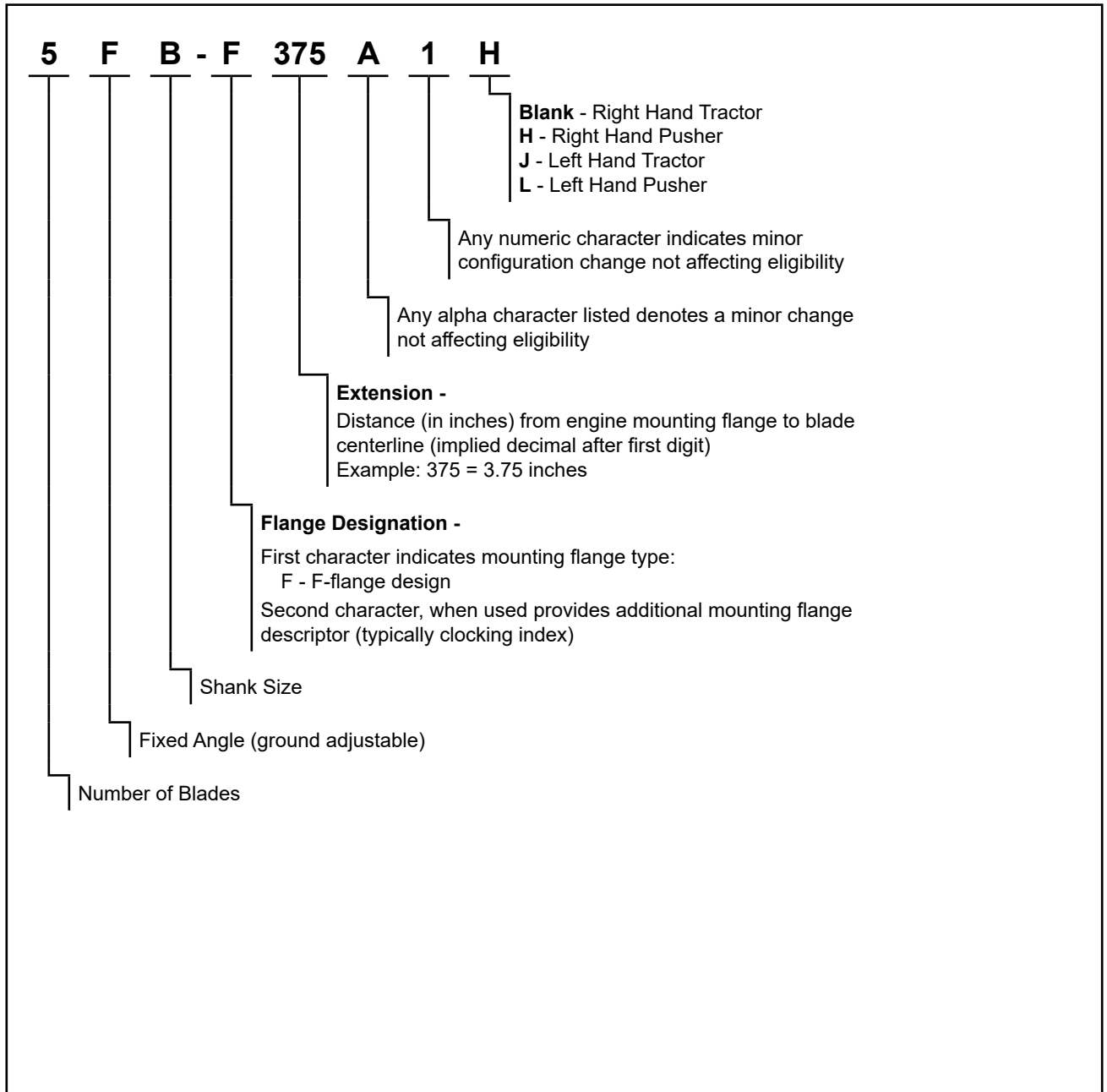
Aluminum Hub Propellers on Reciprocating Engines Identification - Ground Adjustable Series Figure 9
