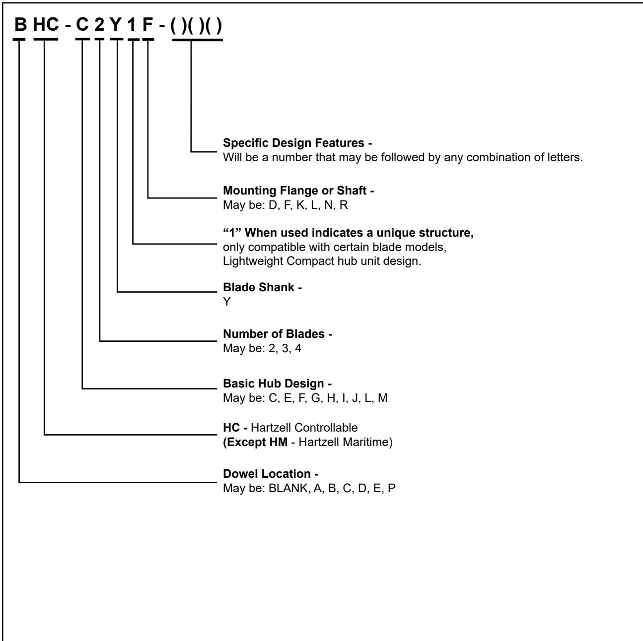
Aluminum Hub Propellers on Reciprocating Engines Identification - Compact Series Figure 3
